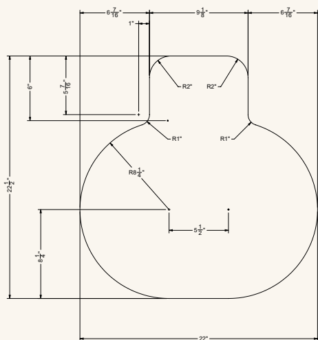
FIG. A Hinge-notch cut-out — plan view
