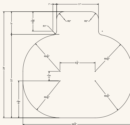
FIG. B Hinge-notch cut-out — plan view
