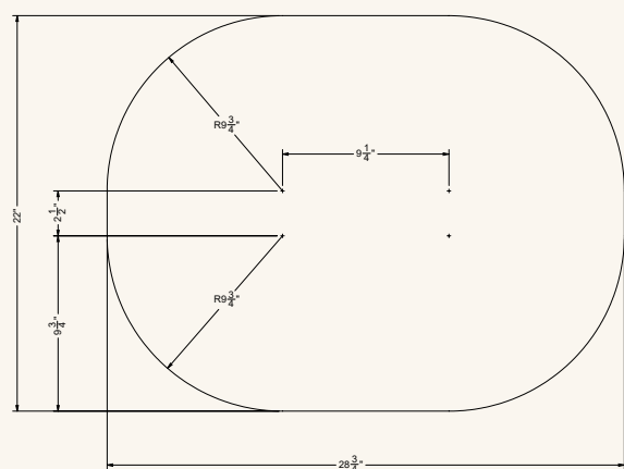
FIG. A Standard cut-out — plan view
