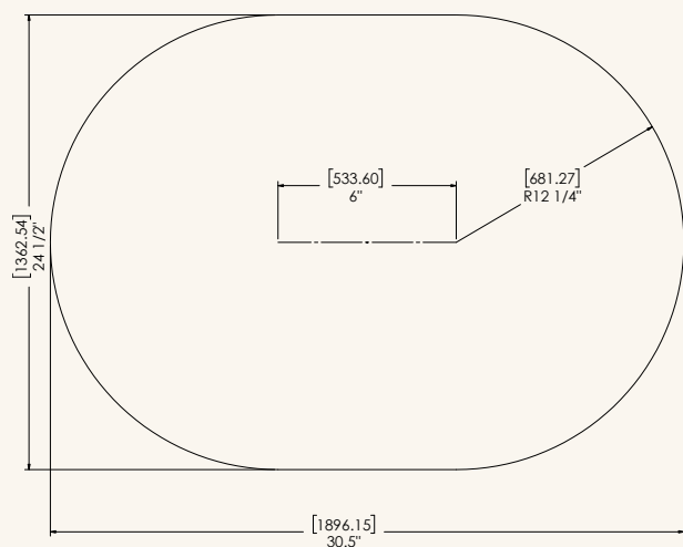
FIG. A Standard cut-out — plan view
